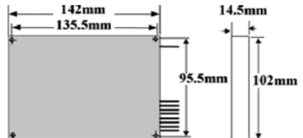
Package E: 14.5mm x 102mm x 142mm
