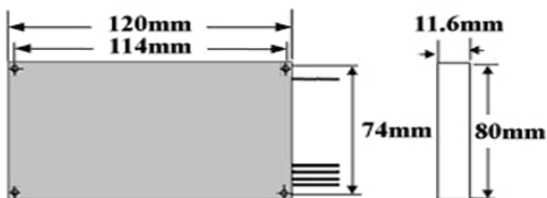
Package D: 11.6mm x 80mm x 120mm
