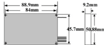
Package S: 9.2mm x 50.88mm x 88.9mm
